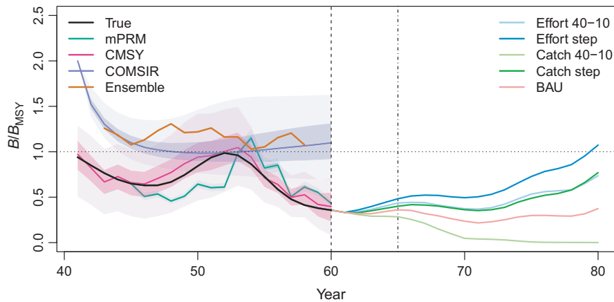
FIGURE 3 An example time series of population status ( B/B_{MSY} ) of corvina reina before and after the catch-only assessment (dotted line: t_{60} ). This example is from the scenario that was simulated with one-way trip effort dynamics (black line). The catch-only assessment was conducted in year 60, assuming only 20 years of catch data were available, using three catch-only models (dark shading = 25th and 75th percentiles, light shading = 2.5th and 97.5th percentiles) and a random forest superensemble to estimate B/B_{MSY} . In this case, the superensemble and COMSIR overestimated stock status, while CMSY and mPRM were more accurate. Projections based on the catch-only assessment show the predicted outcomes from each harvest control rule (HCR) over a 5-year (dash-dot line, t_{65} ) and 20-year management period: effort-based 40-10 HCR, an effort-based HCR set using a step function, a catch-based 40-10 HCR, a catch-based step HCR, and a business as usual scenario (BAU). In this case, the effort-based step HCR was the only strategy that recovered the stock after 20 years
