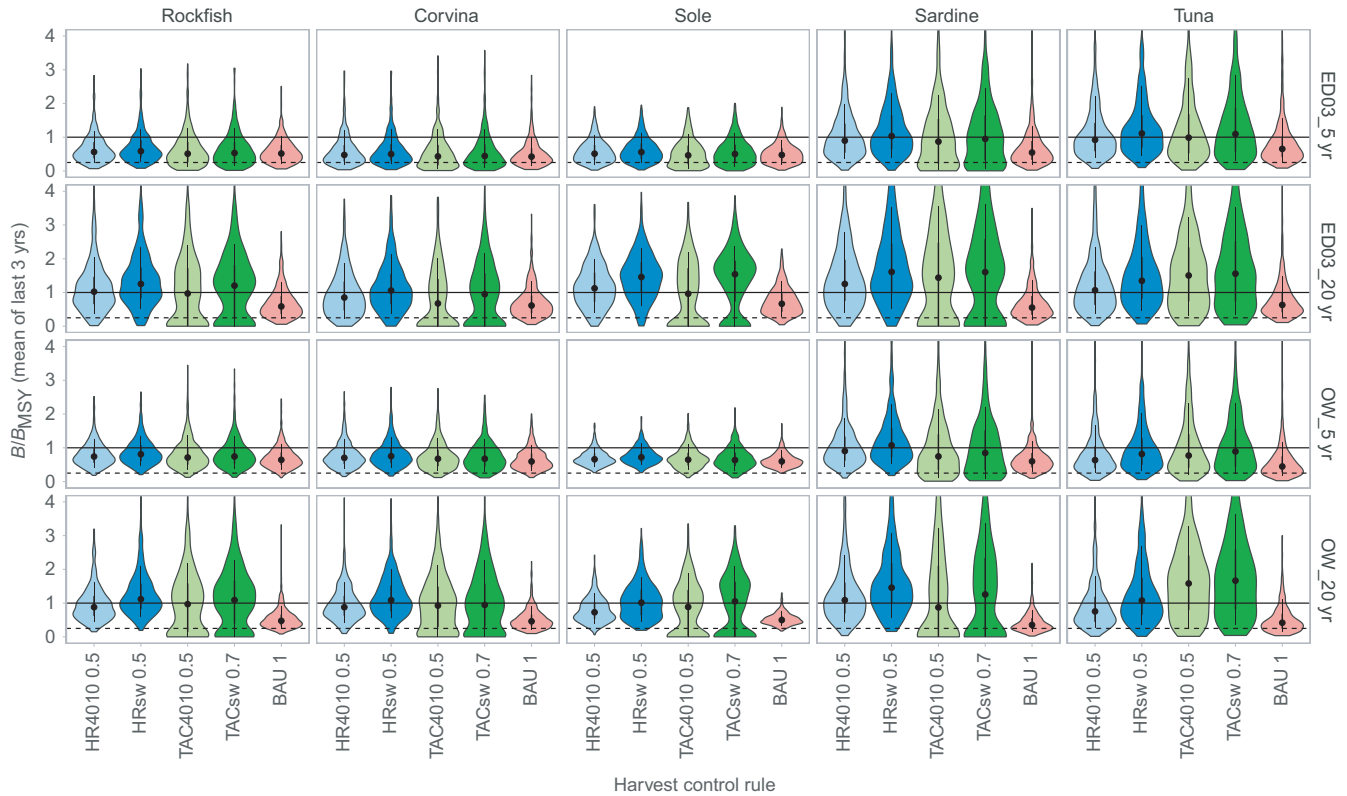
FIGURE 4 Bean plots of fisheries status ( B/B_{MSY} ) after 5 and 20 years of management using each harvest control rule for the one-way trip (OW) and bioeconomic coupling (ED) effort dynamic scenarios (600 iterations per species). Solid line shows B_{MSY} and stocks below the dotted line are heavily overfished ( B/B_{MSY} < 0.25 )
