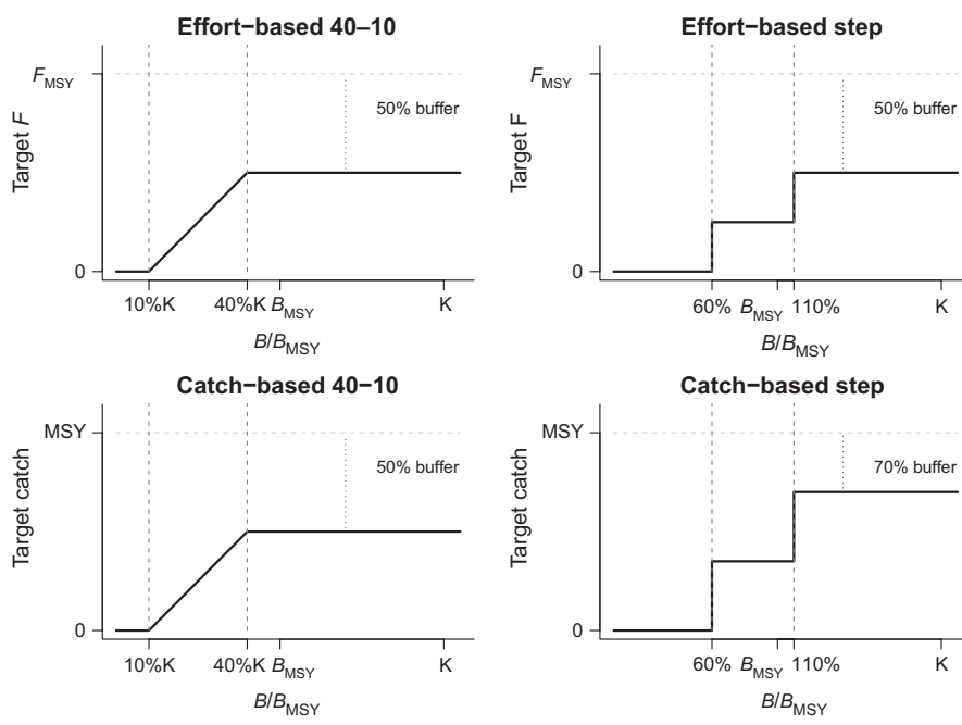
FIGURE 2 Schematics of the 40-10 and step harvest control rules (HCRs) controlling for fishing effort (top panels) or catch (bottom panels). The vertical dashed lines show the trigger and limit points for the 40-10 HCRs (40% and 10% of unfished biomass or carrying capacity, K ), and for the step HCRs (110% and 60% of B_{MSY} ). The vertical dotted line shows the buffers used for each HCR; for example, for the effort-based 40-10 rule, the buffer was 50% F_{MSY}
