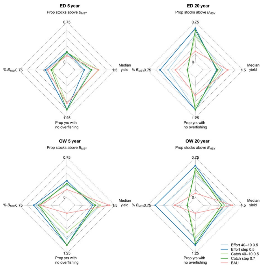
FIGURE 5 Performance of each harvest control rule based on the catch-only superensemble model and calibrated buffers for bocaccio rockfish representing the trade-off between four objectives, clockwise from left corner: (i) lower 10th percentile of B/B_{MSY} status (across iterations, averaged over the last three years of management), (ii) proportion of stocks that were above B/B_{MSY} at end of management period ( B/B_{MSY} > 1 ), (iii) annual median yield over management period across iterations relative to yield if fished at F_{MSY} and (iv) median proportion of years where overfishing was not occurring across the management period ( F/F_{MSY} < 1 ). Each plot shows a different scenario of harvest dynamics and management period, and the results from rockfish are representative of all other species, except tuna shown in Figure 6. All axes have centre values = 0. Each axis along the radar plot displays a different objective, where data points further from the centre of the graph indicate better performance
