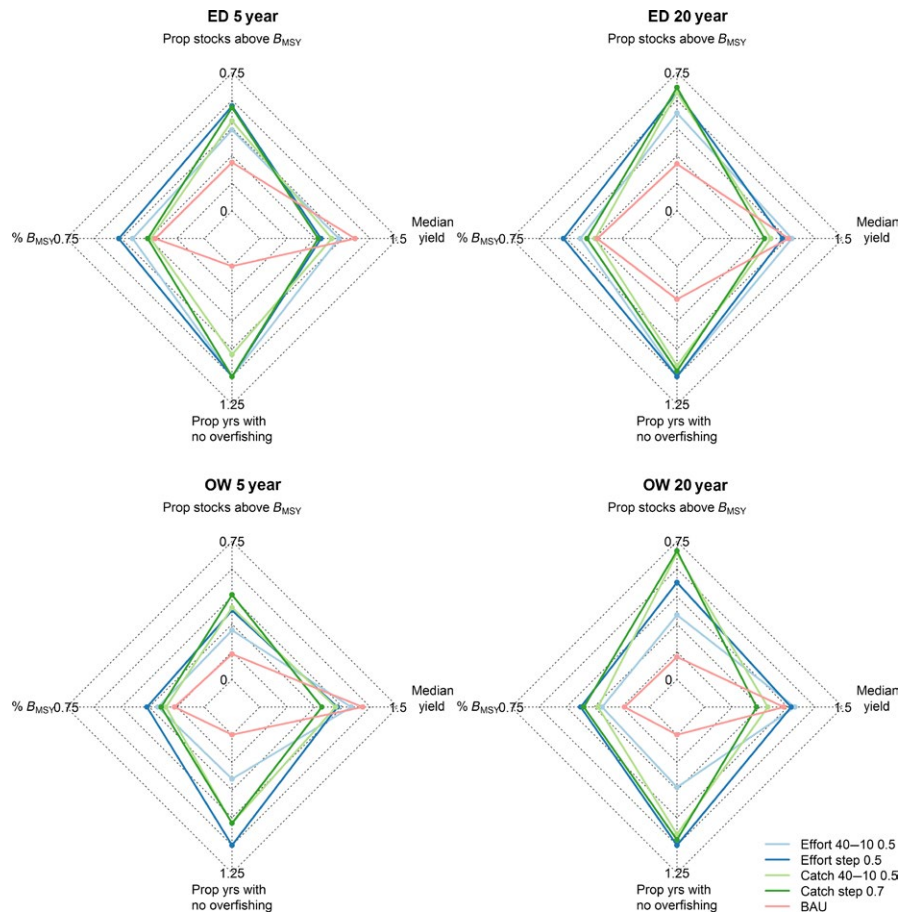
FIGURE 6 Performance of each harvest control rule for skipjack tuna across scenarios, based on the catch-only superensemble model and calibrated buffers representing the trade-off between four objectives clockwise from left corner: (i) lower 10th percentile of B/B_{MSY} status (across iterations, averaged over the last 3 years of management), (ii) proportion of stocks that were above B/B_{MSY} at end of management period ( B/B_{MSY} > 1 ), (iii) annual median yield over management period across iterations relative to yield if fished at F_{MSY} and (iv) median proportion of years where overfishing was not occurring across the management period ( F/F_{MSY} < 1 )
