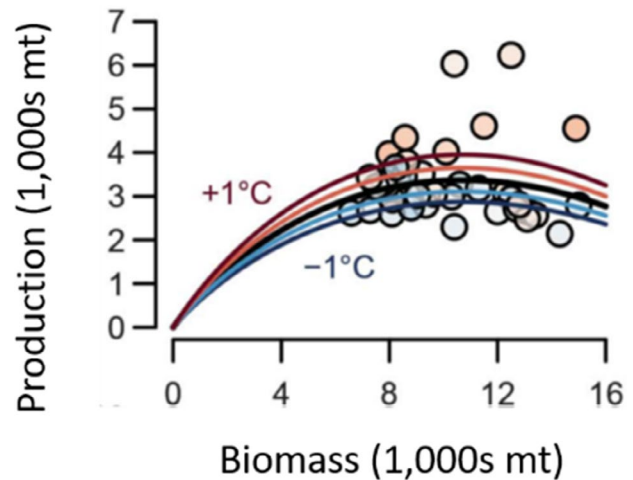
Figure B3. The estimated effect of temperature on the U.S. northern stock of Black Sea Bass. Blue and red points represent cooler- and warmer-than-average years, respectively. Black lines show production at the populations' average temperature. Blue and red lines show production at temperatures progressively cooler and warmer than average, respectively (-1.0°, -0.5°, +0.5°, and +1.0°C). mt = metric tons. Reprinted from Free et al. 2019.
