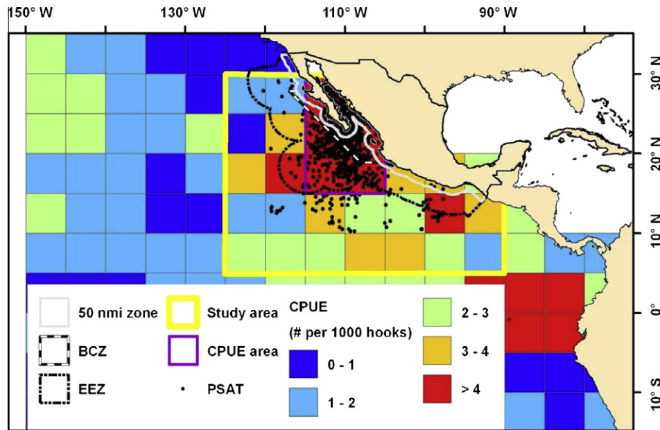
Fig. 3. Striped marlin catch per unit of effort (CPUE, number of individuals 1000 hooks -1 ) from the Japanese long-line fishery averaged over the period 1964–1975. Also shown are Mexico's 50 nautical mile zone (gray), billfish conservation zone (BCZ, black and white dashed), and 200 nautical mile exclusive economic zone (EEZ, black dashed); the study area for the population model (yellow); and the five grid cells near the tip of Baja California from which the commercial CPUE time series was developed (CPUE area, purple). Geolocations (>38 days post-release) of striped marlin tagged with pop-up satellite archival tags (PSAT) are also shown (data from Domeier, 2006).
