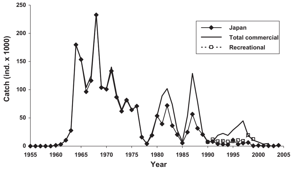
Fig. 1. Catch of striped marlin (1000s of individuals) for the Japanese long-line fleet (solid line and filled diamonds), all long-line fleets combined (thick line), and the recreational fleet based in Cabo San Lucas (open squares and dotted line; Ortega-García et al., 2003).
