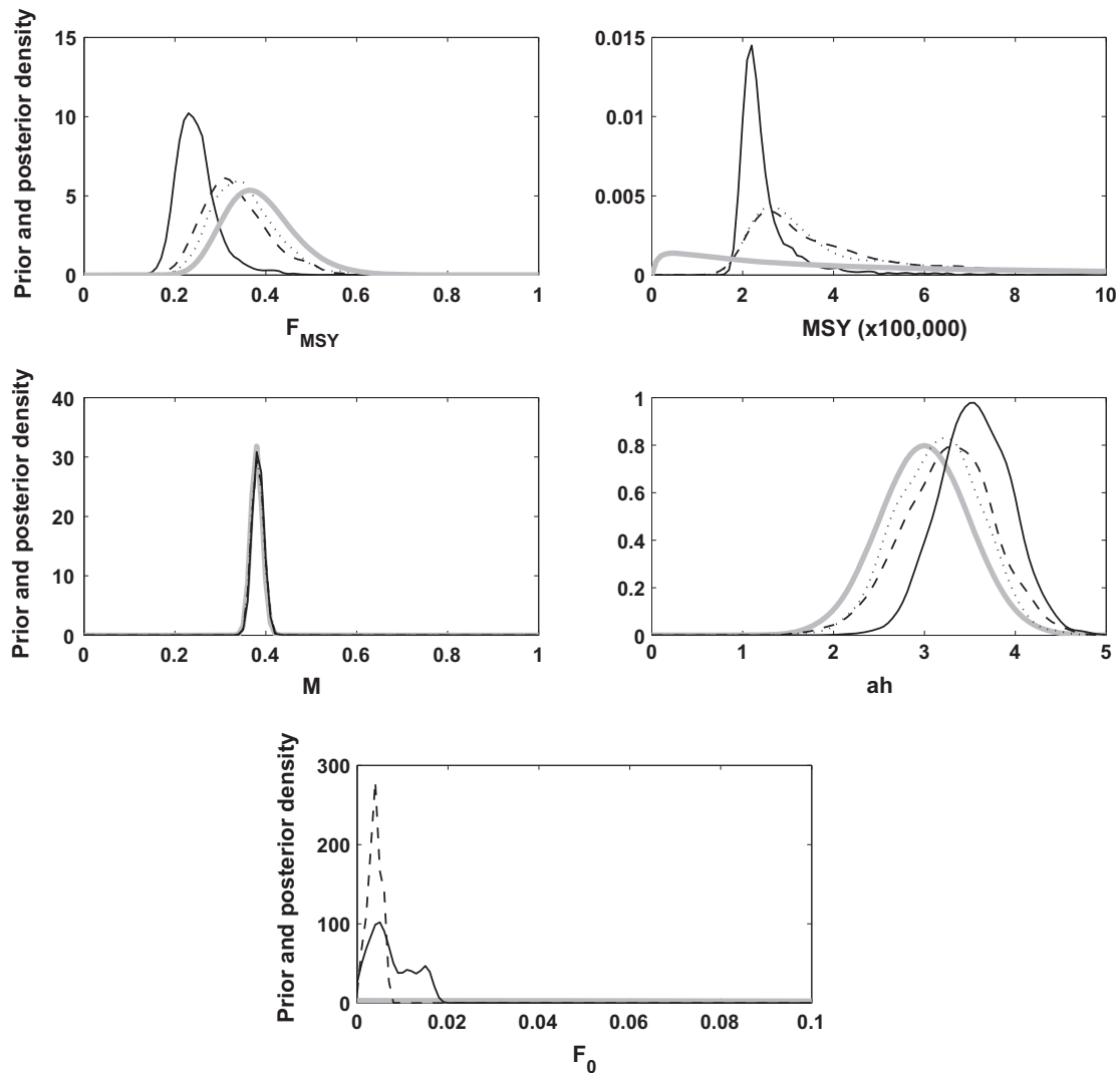
Fig. 7. Normal kernel densities of the marginal posterior distributions (black lines) and the prior distributions (gray line) of model parameters under the deterministic (solid line), 25% process error (dashed line), and 50% process error scenarios (dotted line). Posterior densities are based on 2000 systematic samples from an MCMC chain of length 200,000 where the first 100,000 were discarded to allow for convergence.
