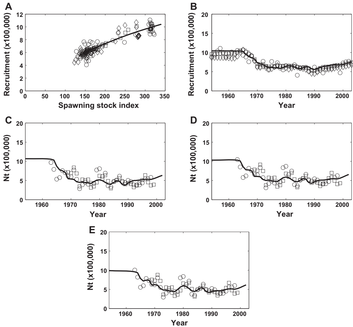
Fig. 8. Stock-recruitment relationship (A) for the deterministic (solid line), Southern Oscillation Index (circles), 25% process error (squares), and 50% process error (diamonds) models; recruitment (age 1) time series (B, same symbols as in A); and modeled vulnerable population size ( N_t \times 100,000 , solid line) for the deterministic (C), 25% process error (D), and 50% process error (E) models. Catch per unit of effort divided by the maximum-likelihood estimate of catchability is shown in C–E for the long-line (circles) and recreational (squares) fisheries.
