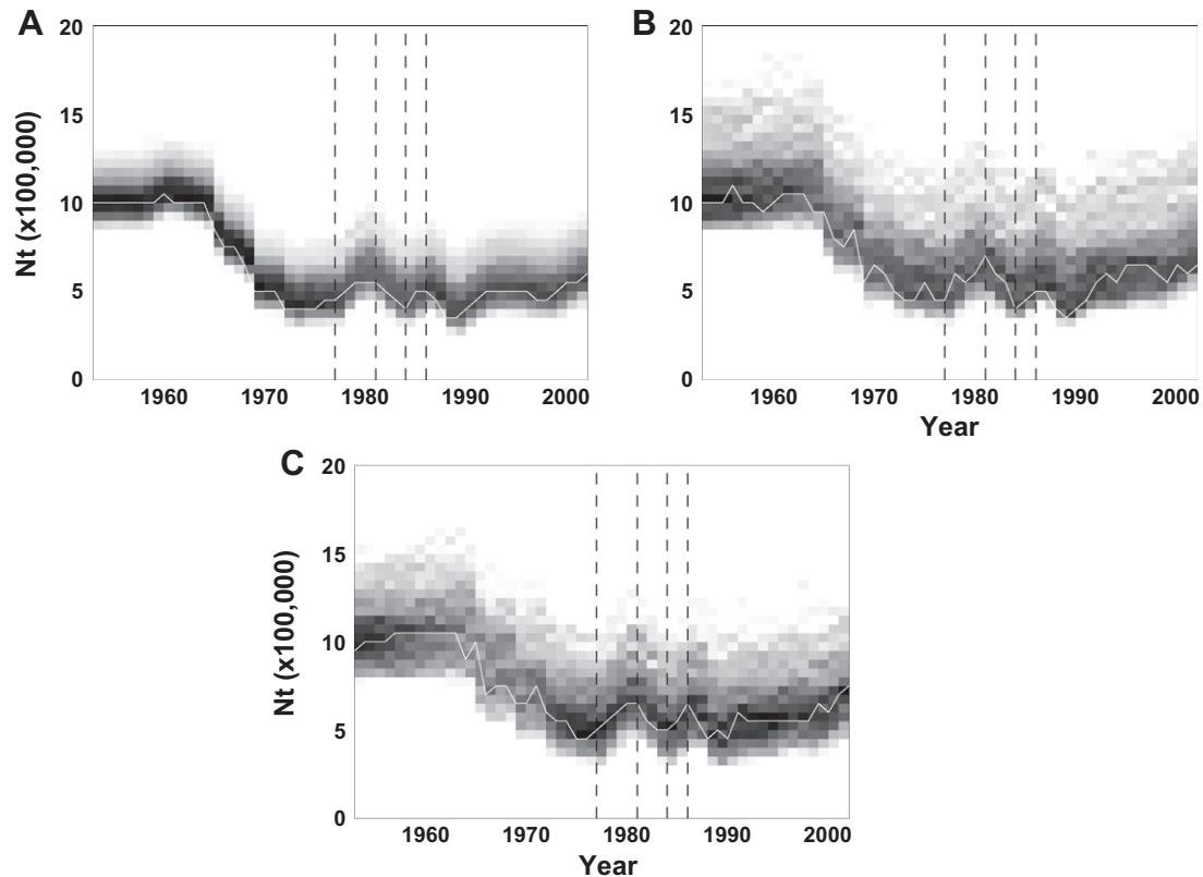
Fig. 4. Time series of modeled vulnerable population size ( N_t \times 100,000 ) for the (A) deterministic, (B) 25% process error, and (C) 50% process error scenarios. High probability values are shown in darker regions, low values in light regions. The white line represents the modal value. Vertical dashed lines denote the two commercial long-line closures.
