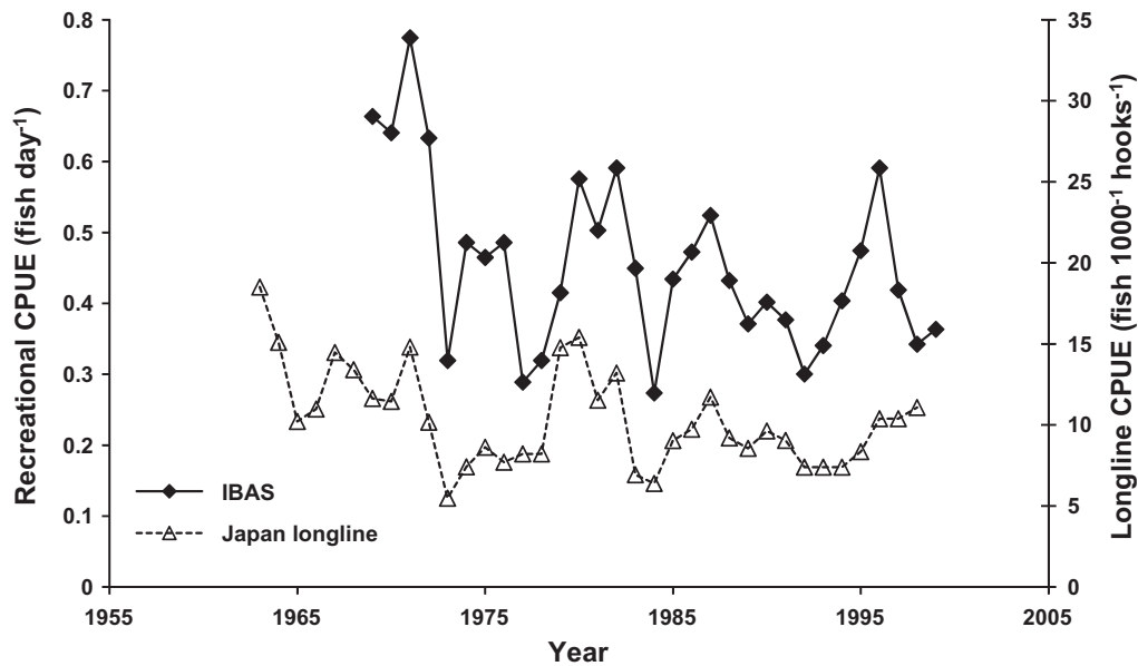
Fig. 2. Catch per unit of effort (CPUE) from the International Billfish Angler Survey (IBAS, filled diamonds, solid line) of anglers fishing near Baja California and catch per unit of standardized effort from the Japanese long-line fishery (open triangles, dotted line) averaged over the five grid cells near Baja California shown in Fig. 3 using the spatial backfilling method of Walters (2003).
