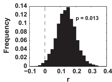
Fig. 6. Marginal posterior distribution of the Pearson correlation coefficient ( r ) between the Southern Oscillation Index (SOI) and recruitment deviations under the deterministic (i.e. observation error only) scenario. Posterior distribution is based on 2000 systematic samples from an MCMC chain of length 200,000 where the first 100,000 were discarded to allow for convergence.
