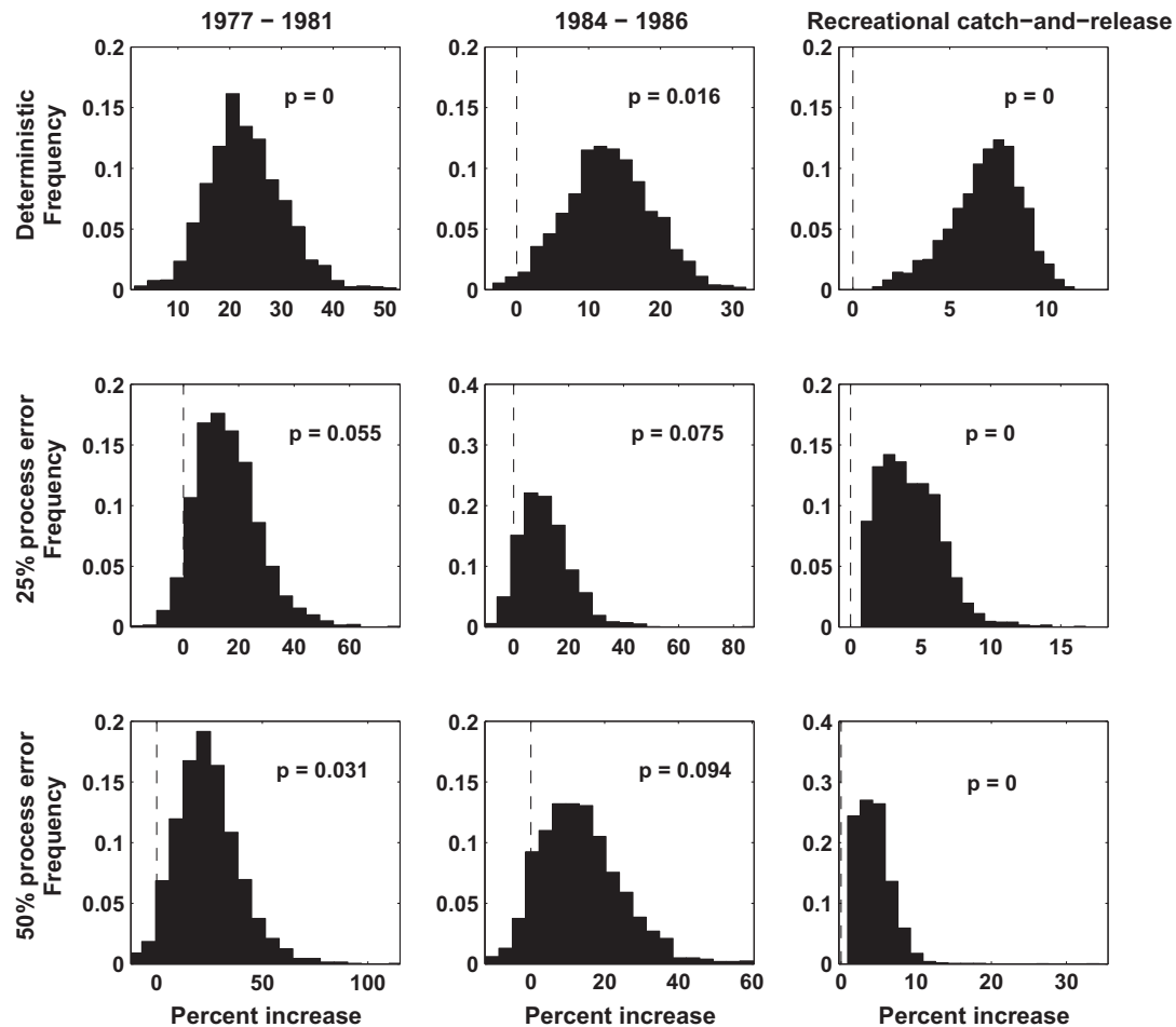
Fig. 5. Marginal posterior distributions for (column 1) the percent increase in vulnerable abundance from 1977–1981 and (column 2) 1984–1986, and (column 3) the percent increase in vulnerable abundance in the year 2000 for strict catch-and-release relative to no catch-and-release during the period 19,901,999. Rows represent (row 1) the deterministic, (row 2) 25% process error, and (row 3) 50% process error scenarios. Posterior distributions are based on 2000 systematic samples from an MCMC chain of length 200,000 where the first 100,000 were discarded to allow for convergence. The proportion of samples for which the percent increase is <0 ( p ) is given in each panel.
